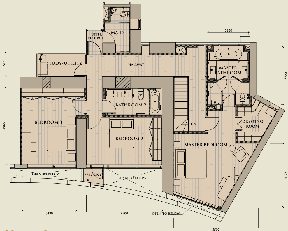
UPPER LEVEL
