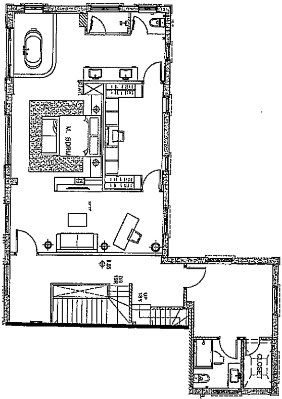
2/F Layout
