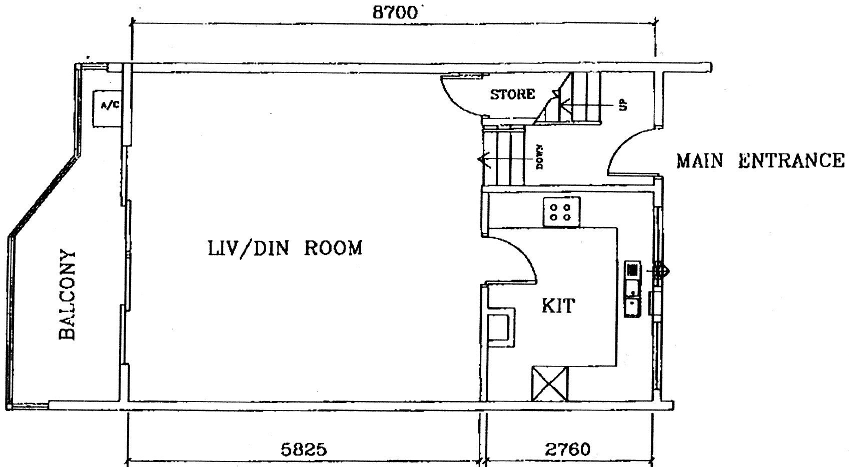
G/F FLOOR PLAN
